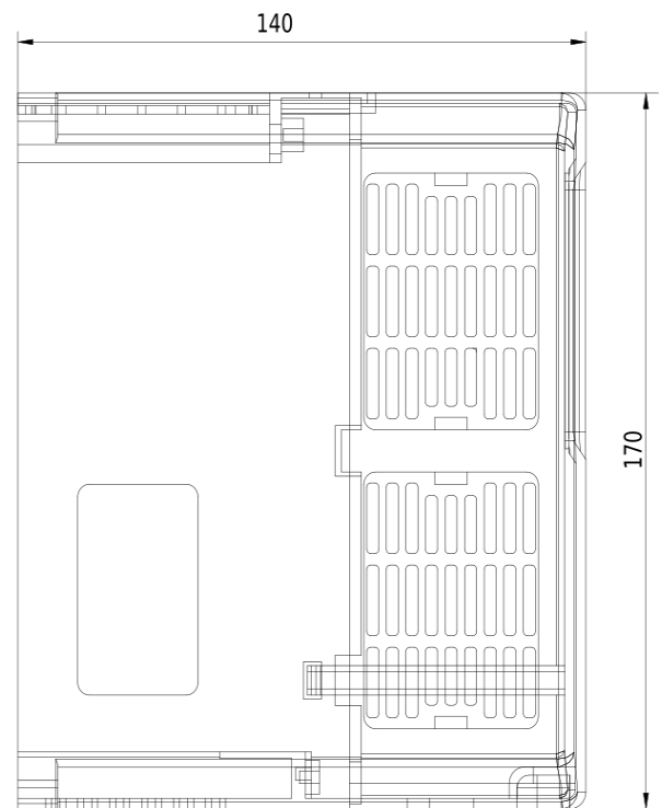
Dimensional drawing V810 - 0,75kW 4T0007
