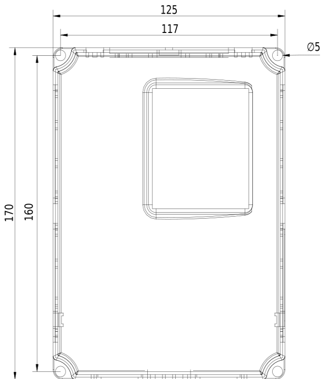
Dimensional drawing V810 - 0,75kW 4T0007
