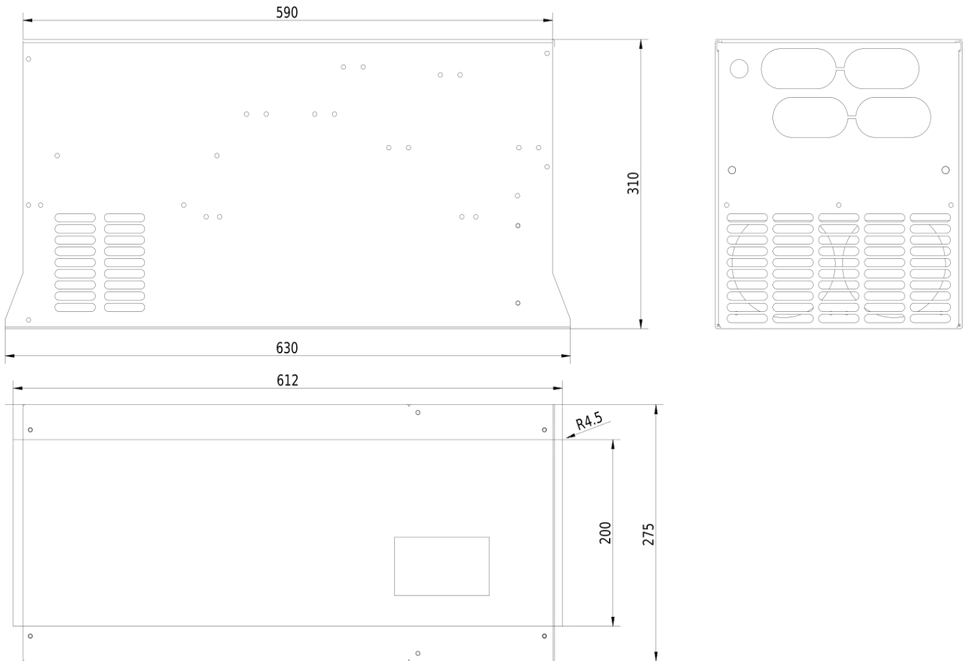
Dimensional drawing V900 - 110kW 4T1100
